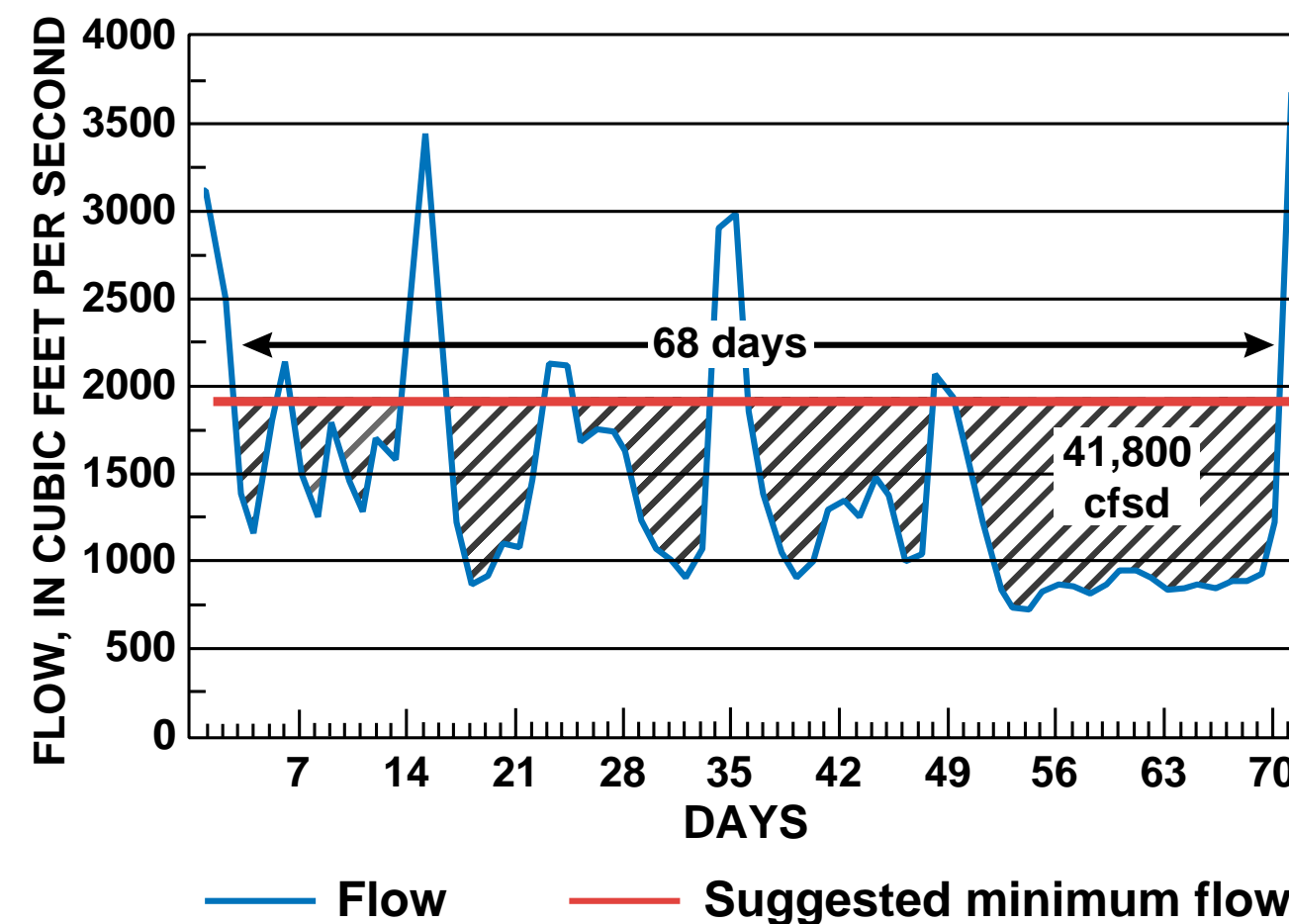
Figure 4. Daily flow of the Pee Dee River at the Pee Dee gaging station during the period August 8 through October 16, 1954, and the minimum flow based on the equation in the State Water Plan.
